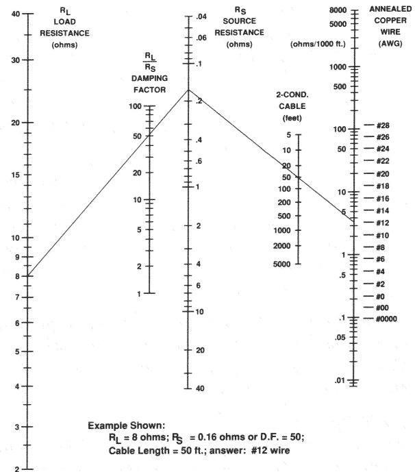
Fig. 3.5 Wire-Size Nomograph
