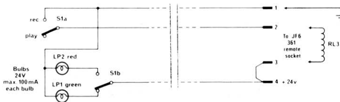
c. Internally powered with indicator
