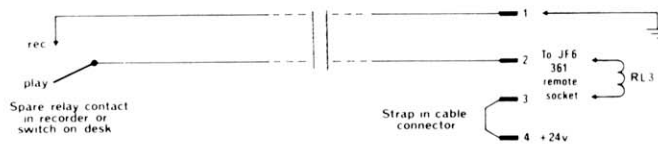
c. Internally powered with indicator
