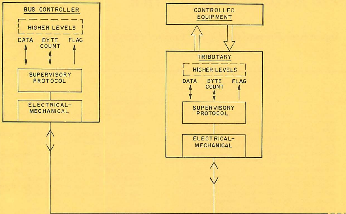
Fig. 1 System Elements
