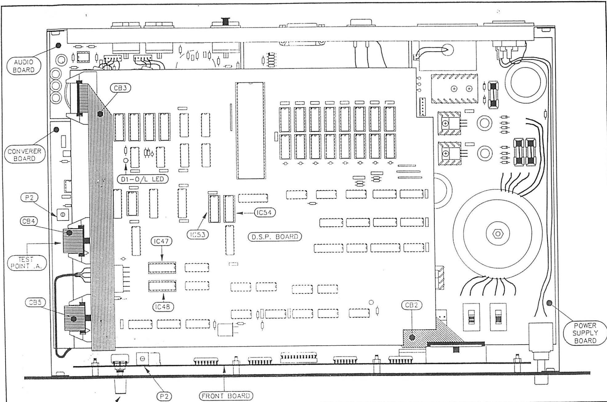
DN780 PLAN VIEW No.2 03.JUN.85
