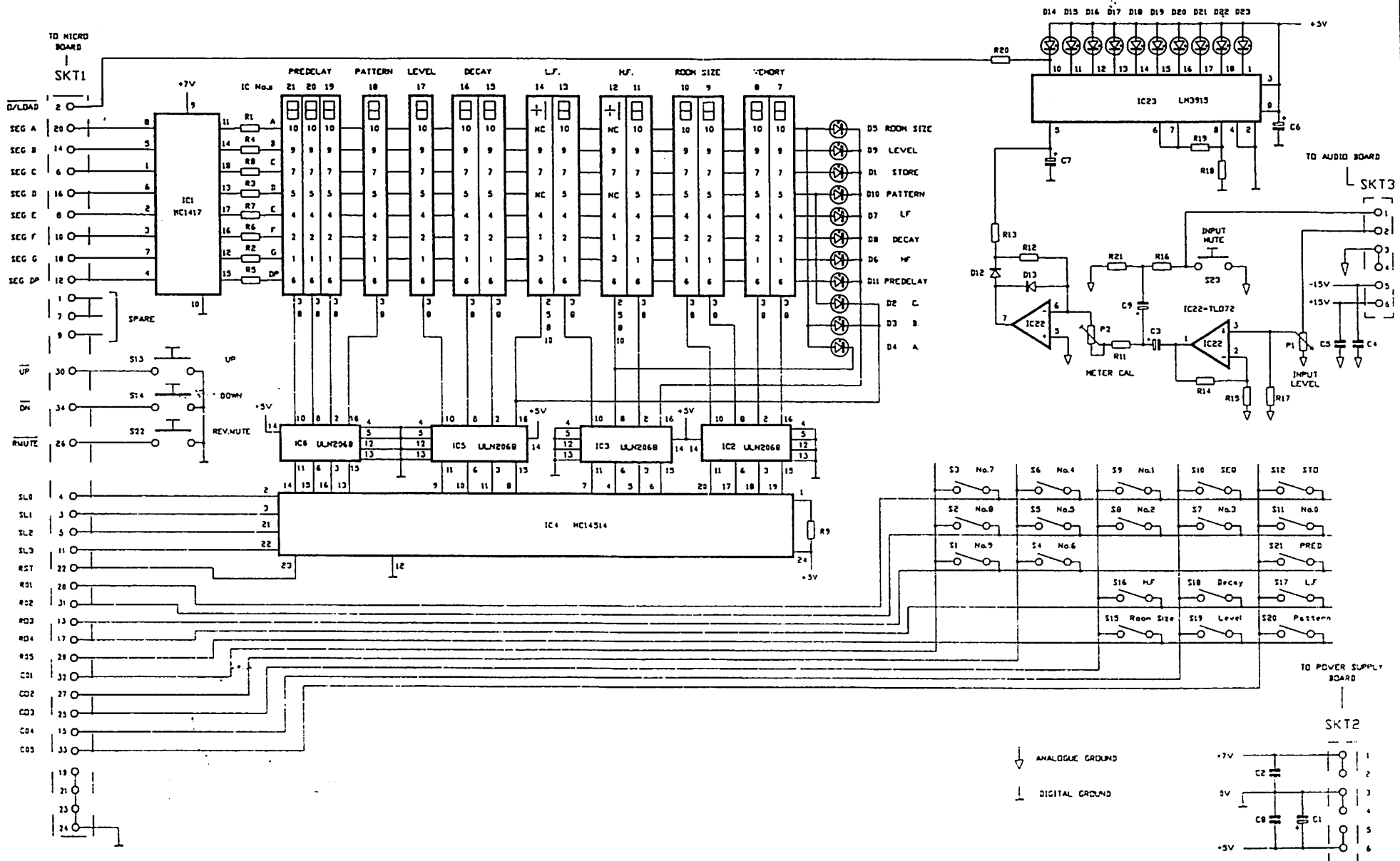
DN780 FRONT PANEL BOARD BRD: 2635/4 27. AUG. 85
