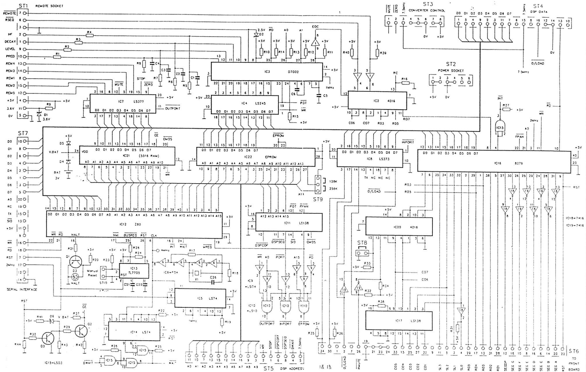
DN780 MICROPROCESSOR SECTION BRD: 2640/3 28 FEB. 85
