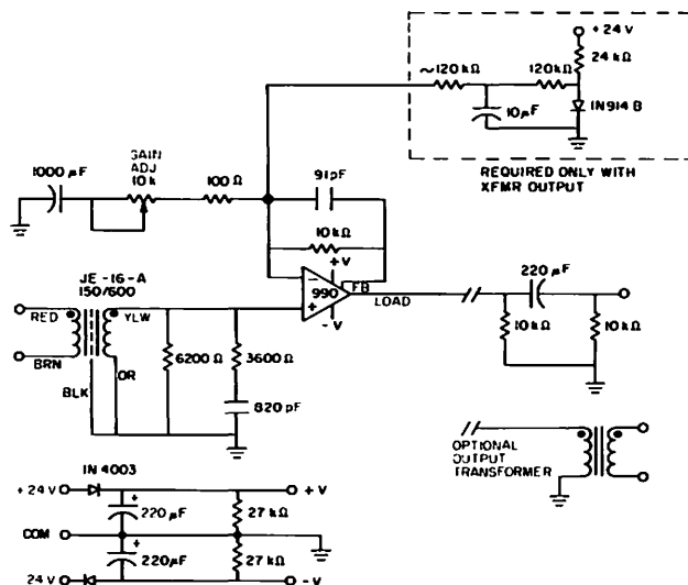
Fig. 13. Microphone preamplifier with offset compensation and adjustable gain.
