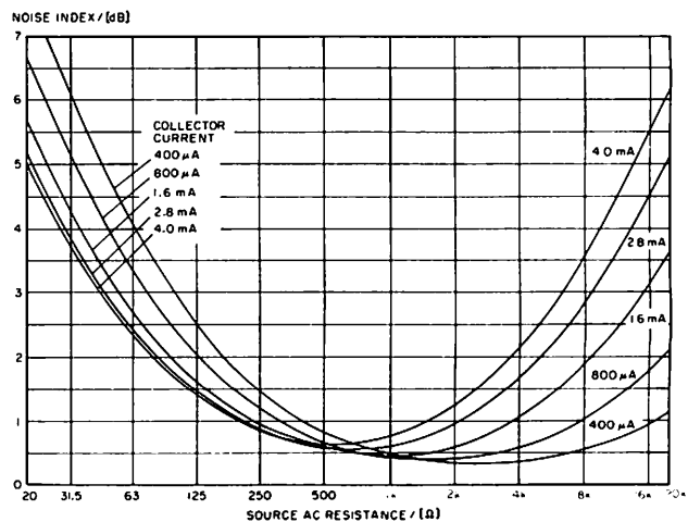
Fig. 4. Noise index versus source ac resistance for a differential pair of transistors, where each transistor is both halves of an LM394 in parallel. Calculated from a measurement in a 20-kHz bandwidth. Parameter: collector current.
